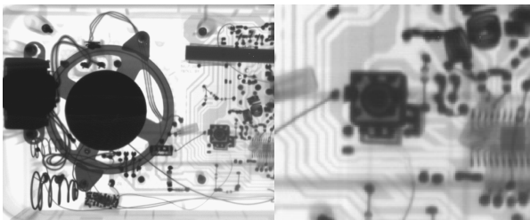
Geometric magnification with microfocus
